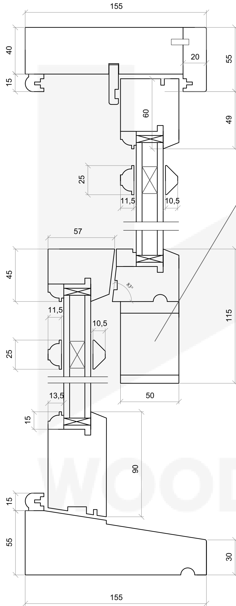
VERTICAL SECTION M1:2
