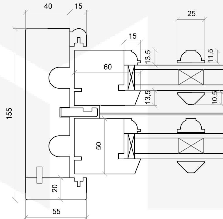
HORIZONTAL SECTION M1:2
