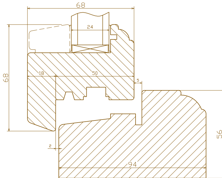
Casement Stormproof window Externally glazed V section
